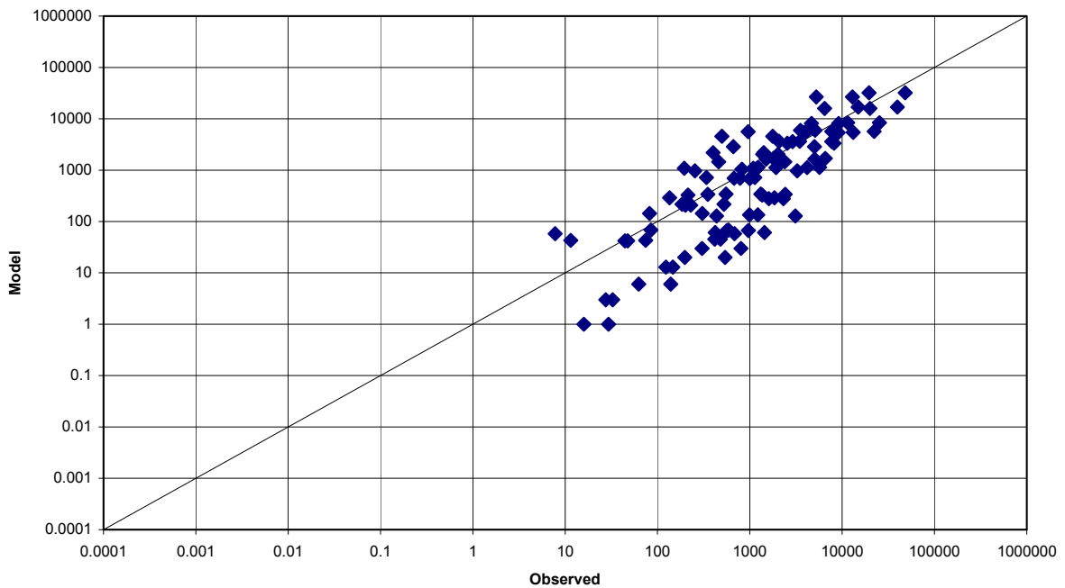
Figure 3. Model vs Observed Off Centerline Concentrations (ppm)
